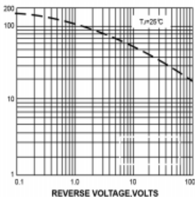
FIG. 5-TYPICAL JUNCTION CAPACITANCE
