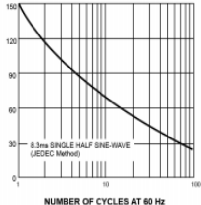
FIG. 2-MAXIMUM NON-REPETITIVE PEAK FORWARD SURGE CURRENT
